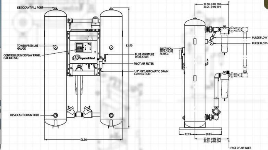
Desiccant Dryer
